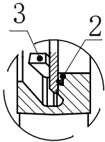
Detail II
